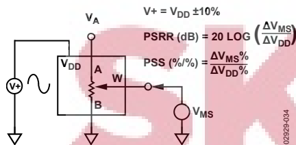
Figure 36. Power Supply Sensitivity (PSS, PSRR)
