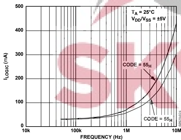
Figure 26. V_{LOGIC} Supply Current vs. Frequency
