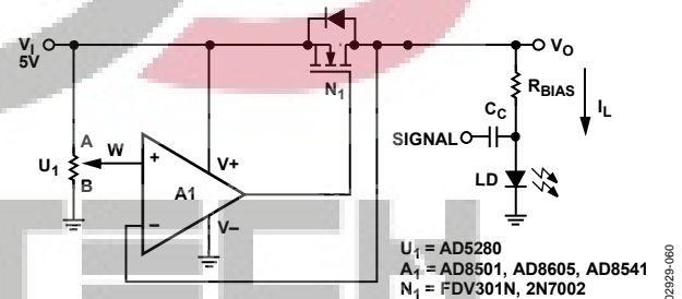
Figure 60. Programmable Boosted Voltage Source
