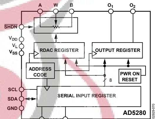
Figure 1. AD5280
