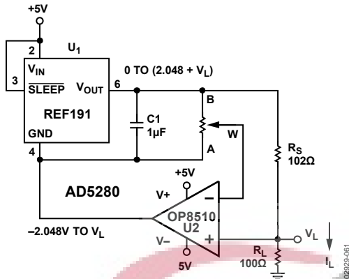
Figure 61. Programmable Current Source
