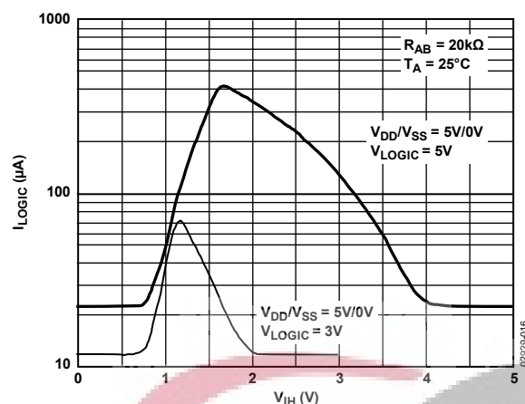
Figure 18. V_{\text{LOGIC}} Supply Current vs. Digital Input Voltage
