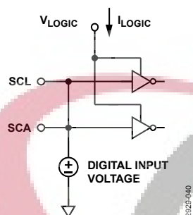
Figure 42. V_{\text{LOGIC}} Current vs. Digital Input Voltage
